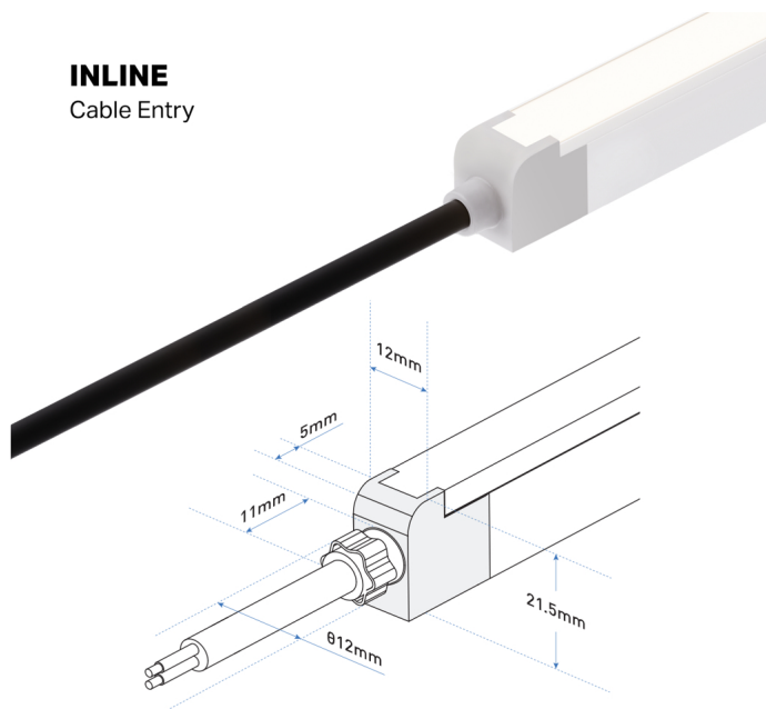
RIGHT / LEFT Cable Entry
